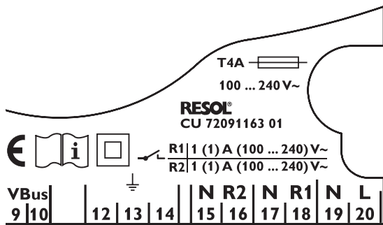
Grounding and load terminals
