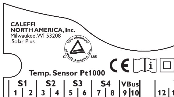
Sensor terminals S1 ... S4
